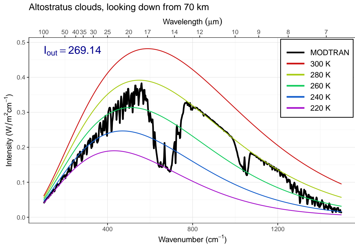
Figure 3: Looking down on altostratus clouds from 70 km
