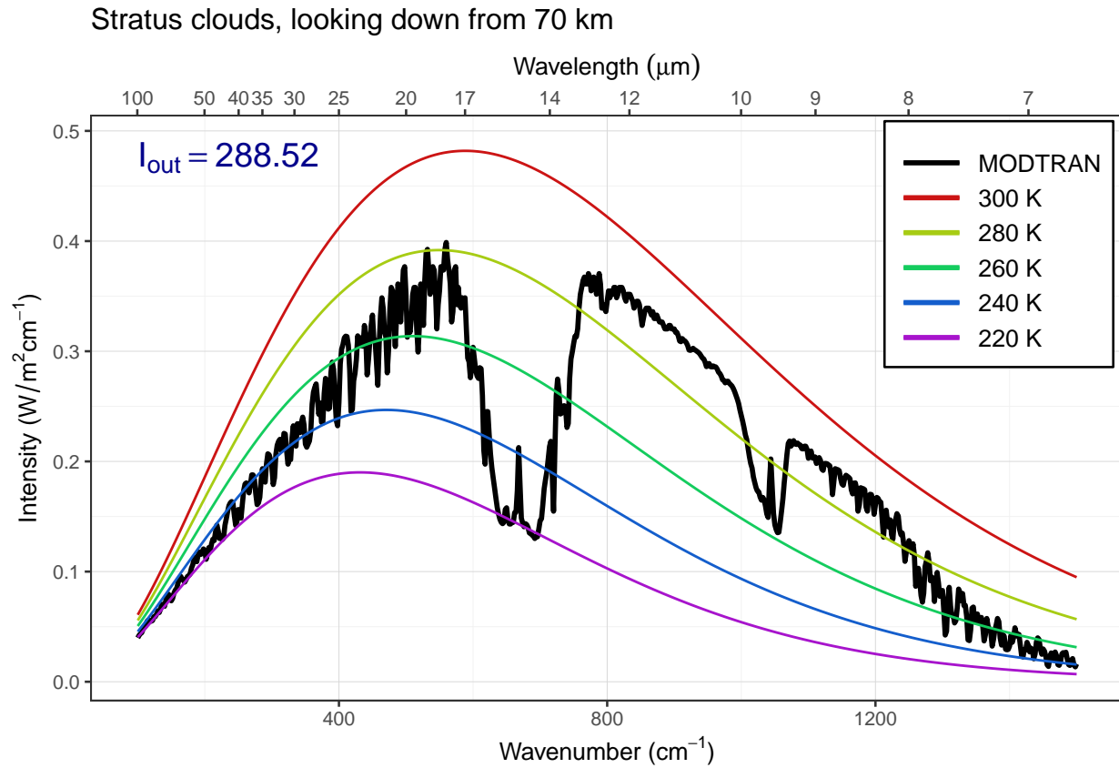
Figure 2: Looking down on stratus clouds from 70 km
